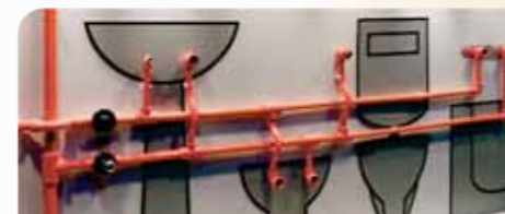
acessórios helitherm pp.r / helitherm blue helitherm pp.r / helitherm blue accessories accessoires helitherm pp.r / helitherm blue accesorios helitherm pp.r / helitherm blue
